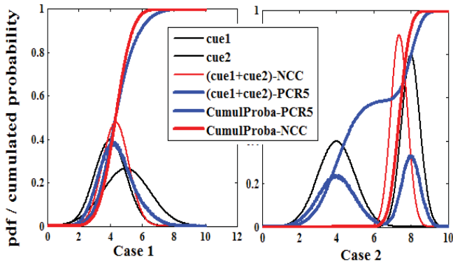
Fig. 1. Performance of pPCR5 fusion rule vs. NCC rule.
