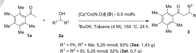
Scheme 3. Gram-scale synthesis.
