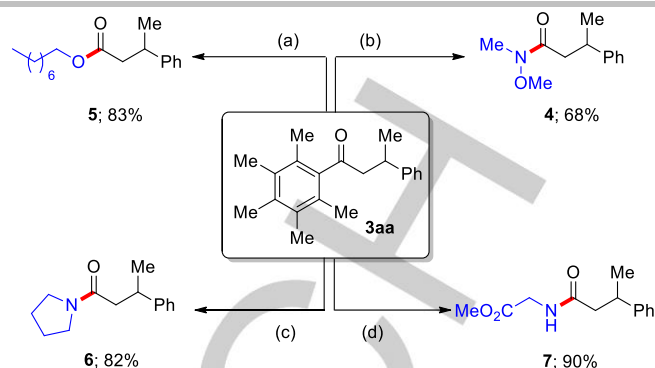
Scheme 5. Diversification of 3aa . Reactions conditions: (a) (i) Br_2 (2 equiv.), CH_2Cl_2 , -17 °C, 15 min (ii) n-octanol (3 equiv.), rt, 20 h; 83% (after 2 steps). (b) (i) Br_2 (2 equiv.), CH_2Cl_2 , -17 °C, 15 min (ii) MeONHMe·HCl (2 equiv.), Et_3N (4 equiv.), rt, 20 h; 68%. (c) (i) Br_2 (2 equiv.), CH_2Cl_2 , -17 °C, 15 min (ii) pyrrolidine (3 equiv.), rt, 20 h; 82%. (d) (i) Br_2 (2 equiv.), CH_2Cl_2 , -17 °C, 15 min (ii) NH_2CH_2COOCH_3 ·HCl (2 equiv.), Et_3N (4 equiv.), rt, 20 h; 90%.
