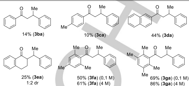
Scheme 2. Effect of substituents on arenes.
