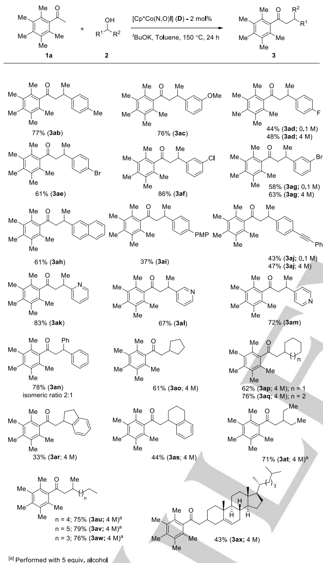
Scheme 4. Scope of secondary alcohols.
