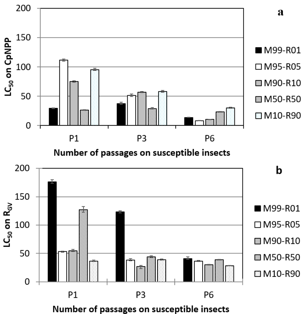
Figure 2. Efficiency ( LC_{50} ) of the different experimental virus populations replicated on CpNPP and tested on (a) CpNPP and (b) R GV . Parental CpGV-M and CpGV-R5 alone had LC_{50} s on CpNPP and R GV of 13.10 OB/ \mu L and 6.76 OB/ \mu L, respectively.
