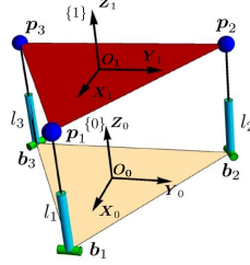
Figure 1: The 3-RPS parallel manipulator
