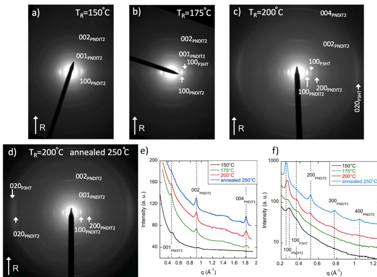
Figure 5. Evolution of the electron diffraction pattern of rubbed P3HT- b -PNDIT2 copolymer films as a function of the rubbing temperature T_R . (a) T_R=150^\circ\text{C} , (b) T_R=175^\circ\text{C} , (c)
