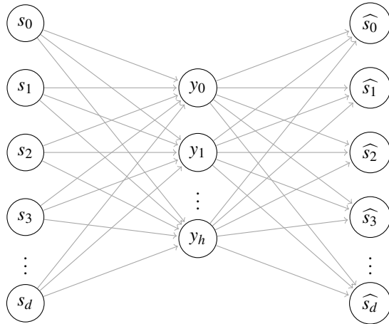
Figure 1. Autoencoder neural network architecture with one layer
