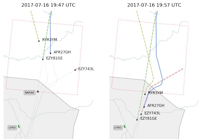
Figure 12. Aircraft are sequenced for landing before entering Toulouse TMA; AFR27GH is vectored behind EYZ81GE and EYZ743L.
