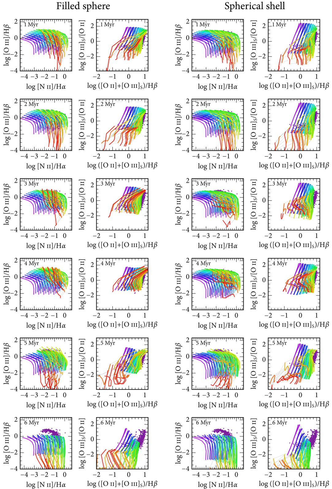
Figure 2. The model grid on [O\ III]/H\beta versus [N\ II]/H\alpha (BPT), and [O\ III]/[O\ II] versus ([O\ II] + [O\ III]_s)/H\beta diagrams for various ages (1–6 Myr) and geometries (filled sphere or empty spherical shell, indicated at the top of the figure). The aim of the postage-stamp size panels is twofold. First, one can see at a glance how the different parameters change the shape of the model subgrids. Secondly, the model grid is overplotted on the observational data, which allows one to judge how well the grid covers the observational points. The fact that most points are hidden behind the grid is thus a fact to be celebrated. The colour-coding of grid lines is detailed in Fig. 3, which zooms into two panels. A colour version of this figure is available in the electronic edition.
