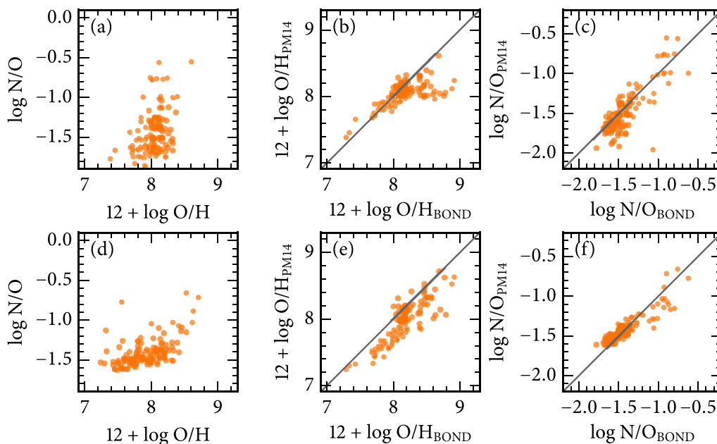
Figure C4. Results for applying the HII-CHI-MISTRY code by Pérez-Montero (2014) to our sample B. Top and bottom rows, respectively, show results excluding or including [\text{O III}]\lambda 4363 from the HII-CHI-MISTRY fits. From left to right, the N/O versus O/H diagram, and the comparison between the O/H and N/O values to BOND.
