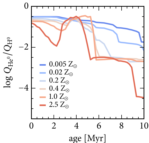
Figure 4. The values of Q(\text{He}^0)/Q(\text{H}^0) as a function of time for the PopStar models at different metallicities. The hardness of the radiation field in an \text{H II} region tends to decrease with age, but the Wolf–Rayet phases wreaks havoc on this simple view.
