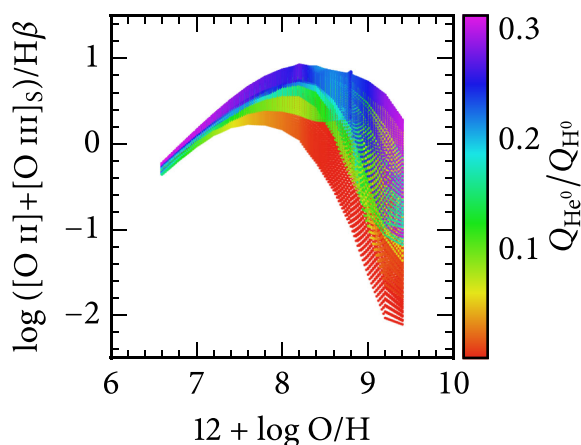
Figure 5. ([\text{O III}]_S + [\text{O II}])/\text{H}\beta versus \text{O}/\text{H} for \log U = -2 and all the values of \text{N}/\text{O} , ages and density structures in our grid coloured by Q(\text{He}^0)/Q(\text{H}^0) . In order to see the trends better, we have created a very fine interpolated grid for this figure (sampled 0.02, 0.05, 0.05 dex in \text{O}/\text{H} , \text{N}/\text{O} and U , respectively). Note that, for high metallicities, the ([\text{O III}]_S + [\text{O II}])/\text{H}\beta ratio does not pin down the value of the \text{O}/\text{H} abundance. A colour version of this figure is available in the electronic edition.
