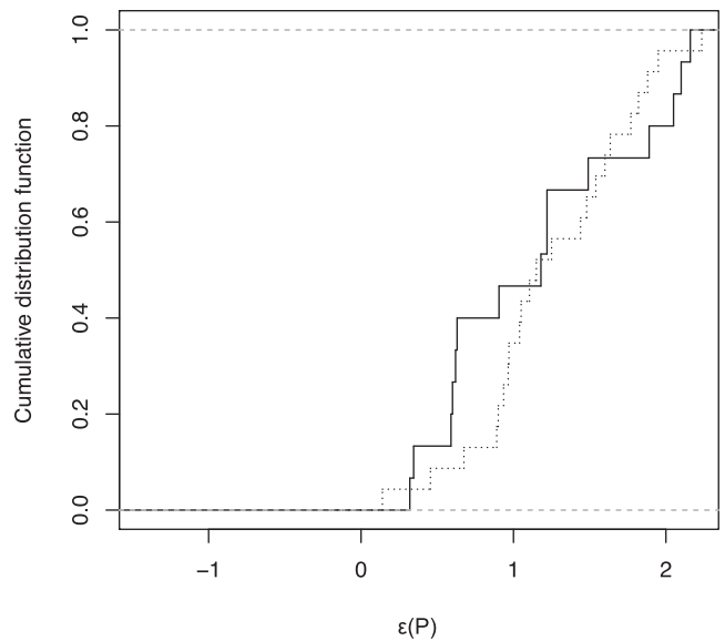
Figure 8. Cumulative distribution function for the two subsamples versus phosphorus abundances. The continuous curve represents the first group of HgMn stars, and the dotted one the second group, respectively.
