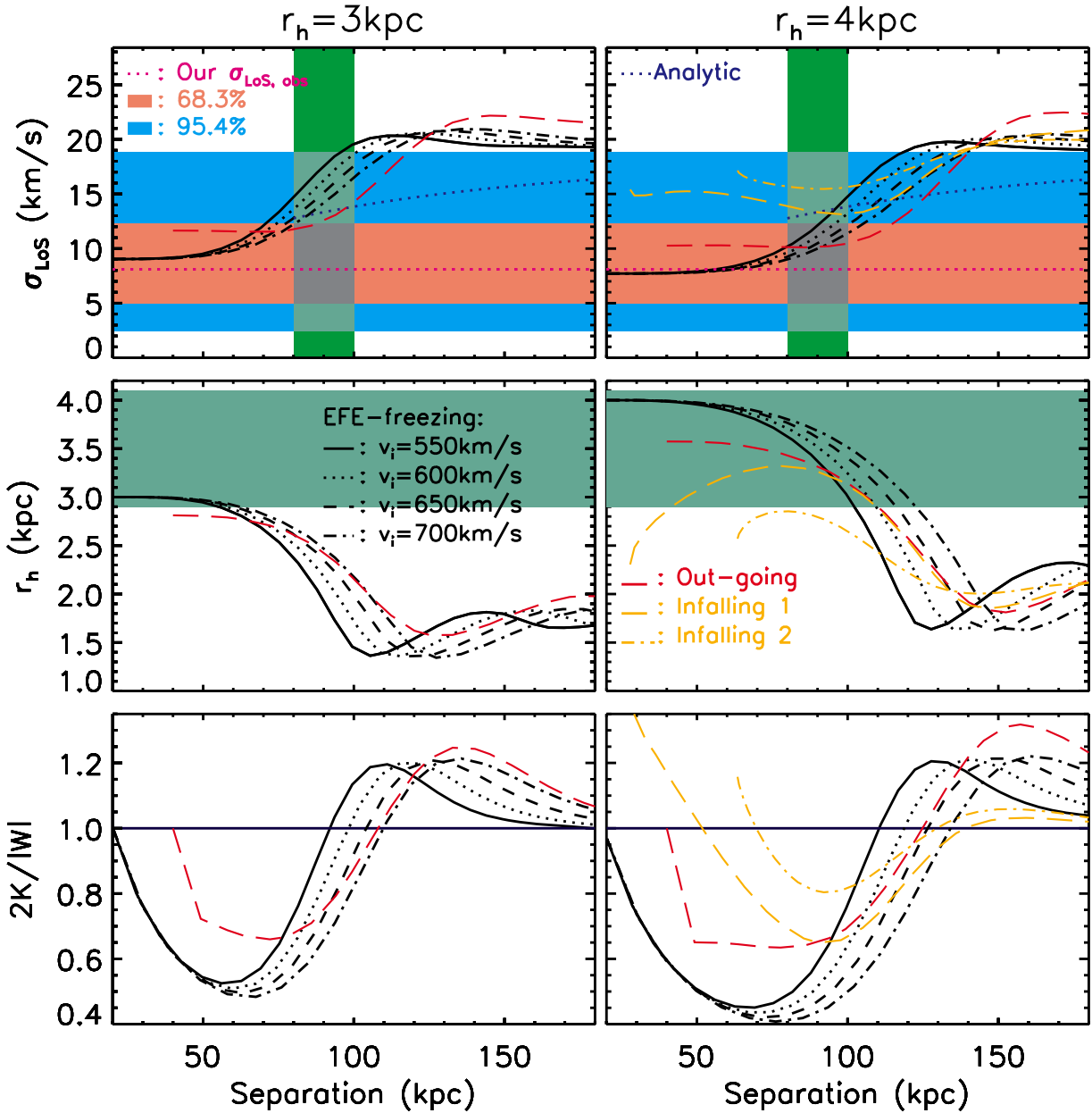
Figure 5. Upper panels: The LoS MOND velocity dispersion \sigma_{M,EF} (equation 1) is shown as a dotted dark blue line in dependence of the separation D_{sep} between DF2 and NGC 1052 for a baryonic mass of M_{NGC1052} = 10^{11} M_{\odot} and D_{sep} > 80 kpc. The vertical green region indicates the expanse between the minimum separation D_{sep} = 80 kpc and the most likely distance D_{sep} = 80\sqrt{3/2} \approx 98 kpc. The 1\sigma and 2\sigma ranges on the here constrained velocity dispersion (Section 3.1), \sigma = 8.0^{+4.3}_{-3.0} km s ^{-1} , are shown as horizontal coloured regions. The analytically calculated velocity dispersion \sigma_{M,EF} (only shown for D_{sep} > 80 kpc) approaches the isolated value \sigma_M = 20 km s ^{-1} asymptotically for large D_{sep} . It declines with decreasing distance and increasing mass because the external field of NGC 1052 suppresses MONDian self-gravity leading to Newtonian behaviour in the case when a_i \ll a_e . For the nominal host mass M_{NGC1052} = 10^{11} M_{\odot} (Bellstedt et al. 2018) and if D = 98 kpc, the MOND velocity dispersion is in agreement within the 2\sigma confidence range of the here measured value. Black lines show the simulated N-MODY LoS velocity dispersion of DF2 as a function of D_{sep} for different orbits with different pericentre velocities. The left-hand panels represent the simulated dwarf model U1 with an initial half-mass radius r_h = 3 kpc and the right-hand panels are for model U2 with r_h = 4 kpc. The PoR simulation results are shown as red and gold lines, with model parameters given in Table 2. Middle panels: The sizes r_h of the simulated dwarfs versus D_{sep} . The horizontal green region lies between 2.9 and 4.1 kpc, being the deprojected half-light radii of the stars and GCs, respectively. Note how the dwarf contracts when it orbits to a larger D_{sep} because its phantom dark matter halo grows as D_{sep} increases and the external field decreases. This causes the internal acceleration to increase towards the isolated MOND value. Lower panels: The simulated evolving virial ratio of the dwarf versus D_{sep} . Values < 1 (below horizontal line) imply a deep-freeze state.
