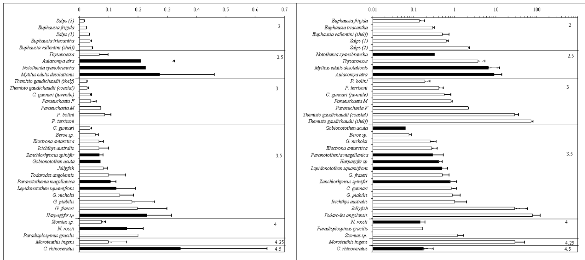
Figure 2 – Hg (left, linear scale) and Cd (right, log scale) concentrations (µg g -1 dw) stratified by trophic level. Benthic species in black, pelagic ones in white.
