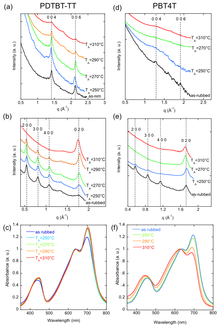
Figure 7. Impact of annealing temperature T_A on the crystalline structure in highly oriented films of PDTBT-TT and PBT4T aligned by rubbing at 200°C. (a) and (d) correspond to the section profile of the ED patterns along the meridian and probe the crystalline order along the chain direction equator. (b) and (e) correspond to the section profile of the ED patterns along the equator and probe crystalline order along the alkyl side chain and/or the \pi -stacking directions. (c) and (f) UV-vis absorption spectra recorded for the polarization parallel to the rubbing direction. The spectra have been normalized in intensity for the 0-1 component to highlight the evolution in the intensity of the 0-0 component as a function of annealing temperature.
