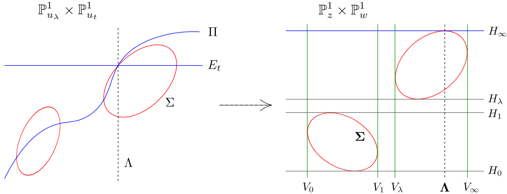
FIGURE 2. Non-generic curves on \mathbb{P}_z^1 \times \mathbb{P}_w^1 and their counterparts in \mathbb{P}_{u_\lambda}^1 \times \mathbb{P}_{u_t}^1 .
