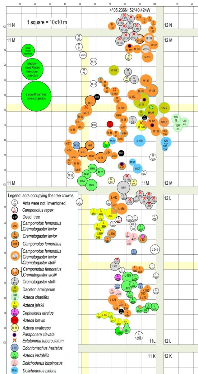
Fig. 2. Overhead view of the distribution of the trees and their associated territorially dominant ant species in the area studied in the Nouragues Ecological Field Station, French Guiana. The codes correspond to the trees listed in Appendix S1 (see also examples of the projection of African tree crowns for comparison).
