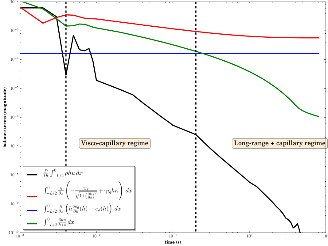
FIGURE 14. Contact line spreading. Time evolution of the magnitudes of the different contributions in the force balance (Eq. (31)) for h_*/h_s = 1/33 . The black dashed vertical lines ( t = 4.0 \times 10^{-3} s and t = 0.2 s) outline the boundaries between the “visco-capillary” and “long-range + capillary” regimes. h_*/\Delta x > 1 .
