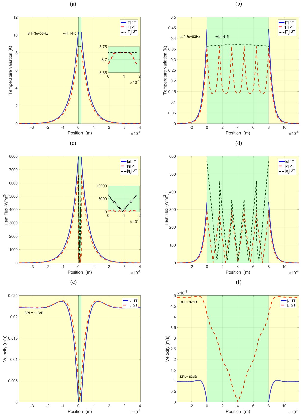
FIG. 4. Near field temperature variations (a,b), heat flux (c,d) and particle velocity (e,f) for a thin (a,c,e) and thick (b,d,f) thermophone. All parameters are plotted only in air with the 1T model and in both air and solid with the 2T model. All curves show the absolute value of the corresponding complex quantities. The central region (green) represents the thermophone layer with both air and solid foam and the regions on the left and on the right (yellow) represent the air layers. The insets in (a) and (c) show a zoom within the generating layer.
