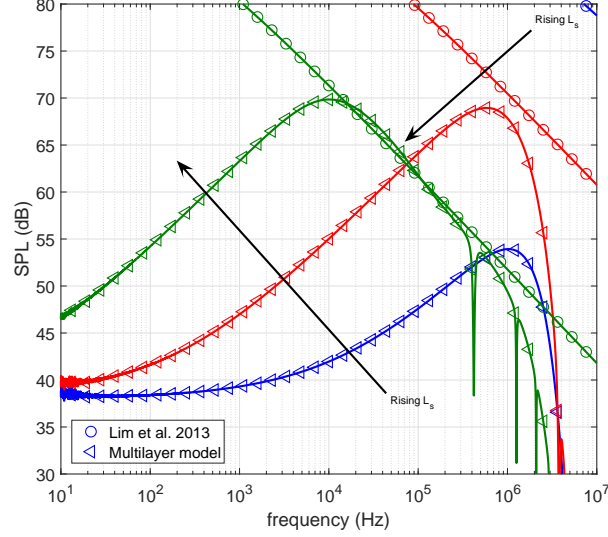
Figure 11: Frequency response of a thermophone with increasing thickness L_s in contact with a semi-infinite substrate on the left and propagating in air on the right (see the scheme in Fig.6). We compare the results of our multilayer model with Eq.(62), describing the free field thermophone [25] .
