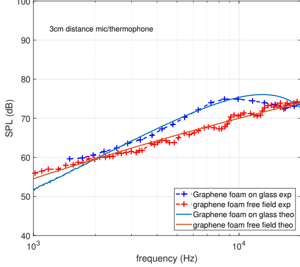
Figure 16: Experimental and theoretical frequency responses of FDGF thermophones. Both the free field case and the geometry with substrate have been considered. The free field case is well described by the relation SPL \sim f^{0.75} , which can be compared with MWNT and ITO-PAN thermophones shown in Fig.15.
