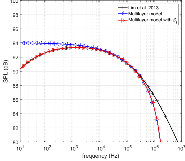
Figure 4: Frequency response of the thermophone in free field determined by means of the Lim et al. model [25] and our multilayer model. We plotted here the results for \beta_s = 28.9 and we also shown the response obtained through the multilayer model with \beta_s = 0 for comparison.
