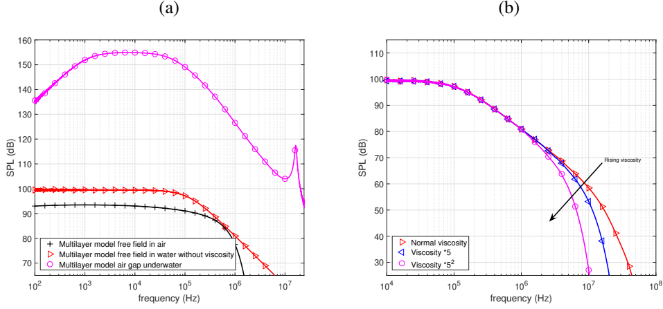
Figure 20: Frequency response of a thermophone working underwater. Panel (a): we can compare the response of the underwater thermophone in free field without viscosity, the underwater thermophone with air gap (e.g. due to hydrophobicity as observed for carbon nanotubes), and finally, the thermophone working in air and in free field. Panel (b): response of the free field thermophone with the normal viscosity of water and two larger values of viscosity.
