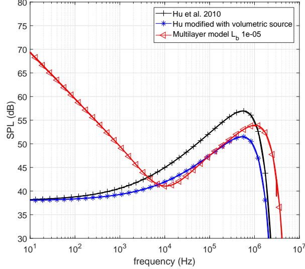
Figure 9: Frequency response of a thermophone placed on a substrate with finite thickness and radiating in air (see scheme in Fig.8). We compare the result of our multilayer model with Eq.(65) [20] and Eq.(66).
