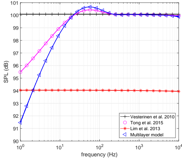
Figure 14: The same plots of Fig.13 for a structure shown in Fig.12, where the substrate is now infinitely large and the air gap size is more than ten times larger. In this case, our result and the Tong’s model [26] achieve the SPL upper bound predicted by Vesterinen [28], corresponding to a 6dB improvement with respect to the Lim’s free field model [25].
