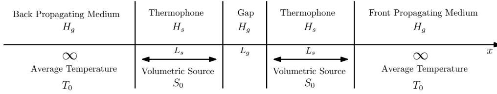
Figure 17: Schematic of a sound generation system composed of two thermophone layers placed in air, separated by an air gap, and radiating symmetrically in both directions.
