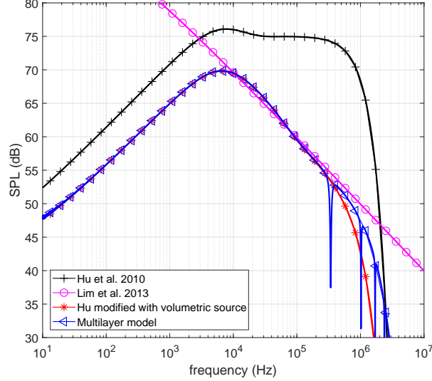
Figure 10: Frequency response of a thermophone in contact with a semi-infinite substrate on the left and propagating in air on the right (see the scheme in Fig.6). The thermophone is here a hundred time thicker than in previous plots. We compare the result of our multilayer model with Eq.(62) by Lim et al. [25], Eq.(65) by Hu et al. [20] and Eq.(66) (modification with volumetric source).
