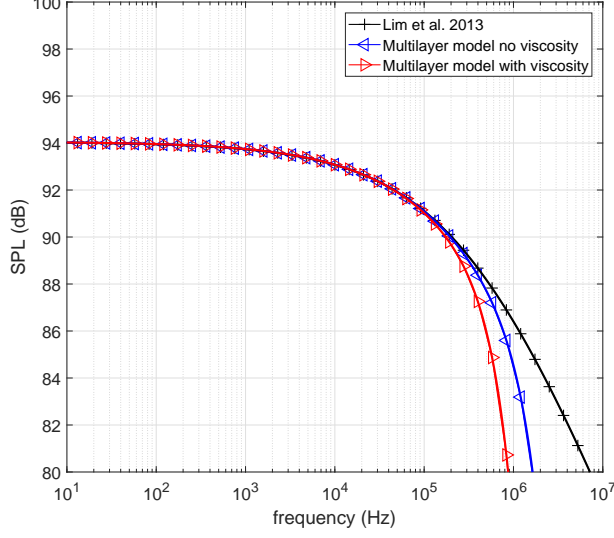
Figure 5: Frequency response of the thermophone in free field determined by means of the Lim et al. model [25] and our multilayer model. We plotted here the results for \beta_s = 0 at a distance of 5 cm, and we introduced the air viscosity in our model to show its effect at high frequency.
