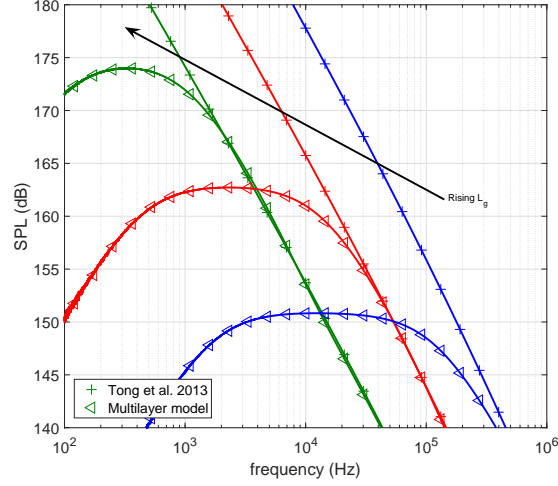
Figure 21: Frequency response for the underwater thermophone with symmetric air gaps. We can find the responses for three different air gap widths and we compare our results with those of Eq.(75), proposed by Tong et al. [31]. We underline the good agreement for the high-frequency behavior.
