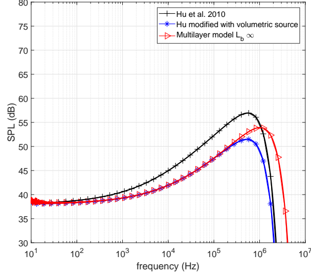
Figure 7: Frequency response of a thermophone in contact with a semi-infinite substrate on the left and propagating in air on the right (see the scheme in Fig.6). We compare the result of our multilayer model with Eq.(65) [20] and Eq.(66).
