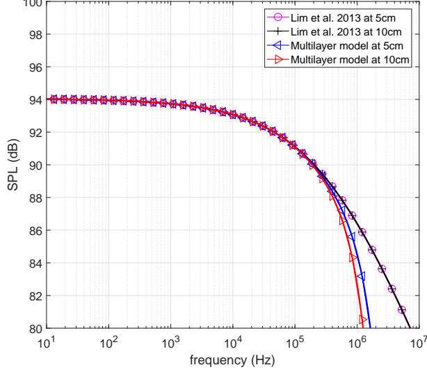
Figure 3: Frequency response of the thermophone in free field determined by means of the Lim et al. model [25] and our multilayer model. We plotted here the results for \beta_s = 0 and for two different observation distances.
