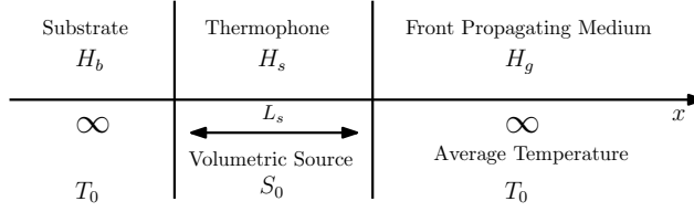
Figure 6: Schematic of a thermophone placed on a solid substrate on the left and radiating in free field on the right. The plane waves are non-symmetrically generated within the back and the front media.
