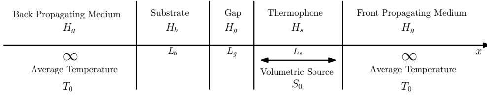
Figure 12: Schematic of a thermophone placed on a solid substrate of finite thickness on the left, and radiating in free field on the right. The plane waves are non-symmetrically generated within the back and the front media.
