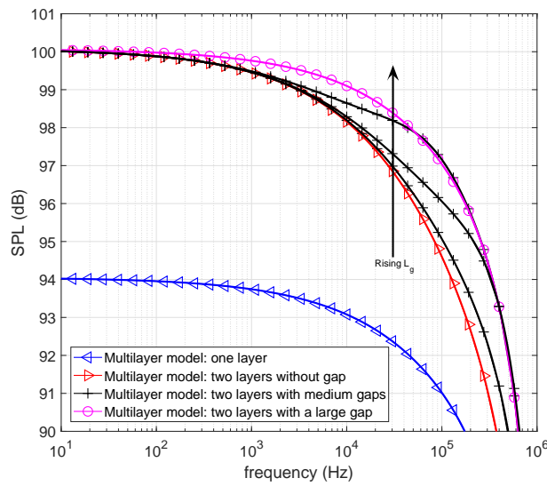
Figure 18: Frequency response of a thermophone system composed of two generating layers separated by a given air gap (see Fig.17 for details). We considered the case without gap L_g = 0 , the case with medium gaps L_g = 1/36, 1/12, 1/4 \times 10^{-4} m, and the case with a large gap L_g = 1 \times 10^{-4} m (independent non-interacting layers). We can observe the effect of the air gap width and compare the result with the single layer thermophone system.
