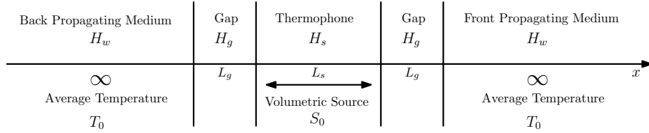
Figure 19: Schematic of a thermophone placed in water by means of two symmetric air gaps, and radiating symmetrically in both directions.
