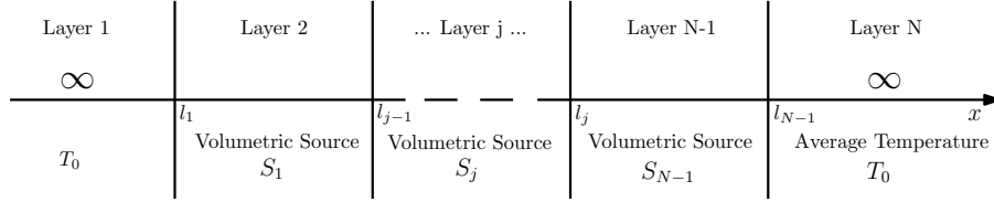
Figure 1: Schematic of a multilayered structures composed of an arbitrary sequence of fluid and solid layers, able to represent different thermoacoustic sound generation systems. While the first and the last regions are semi-infinite, the others correspond to limited layers between l_{j-1} and l_j, \forall j = 2, \dots, N-1 .
