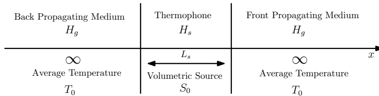
Figure 2: Schematic of a thermophone radiating in free field. The plane waves are symmetrically generated within the back and the front media.
