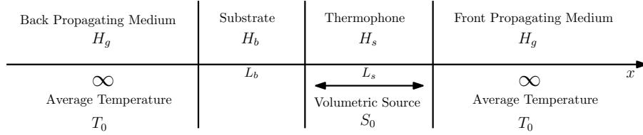
Figure 8: Schematic of a thermophone placed on a solid substrate of finite thickness on the left, and radiating in free field on the right. The plane waves are non-symmetrically generated within the back and the front media.
