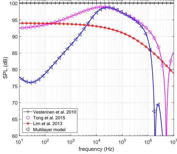
Figure 13: Frequency response of a thermophone placed over a substrate with an air gap, as shown in Fig.12. The result of the multilayer model can be compared with Eq.(71) (Tong et al. [26]). Moreover, we reported the result of the free field model given in Eq.(62) (Lim et al. [25]) and the Vesterinen et al. [28] upper bound reported in Eq.(70).
