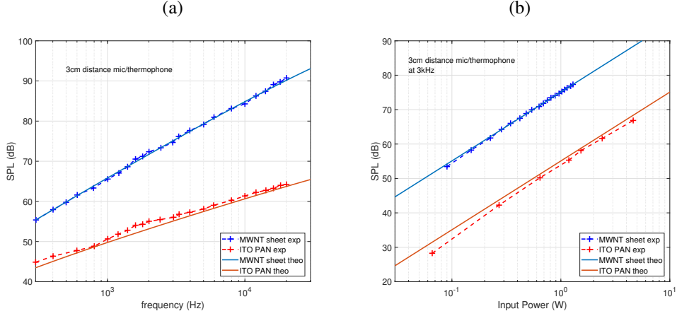
Figure 15: Comparison between the thermoacoustic performances of carbon MWNT sheets and ITO-PAN sheets (experimental and theoretical results). Panel (a): frequency response of the two materials showing the behaviors SPL \sim f^{1.0} for MWNT and SPL \sim f^{0.53} for ITO-PAN (the plots correspond to a normalized power of 1W). Panel (b): SPL versus input power for the two materials.
