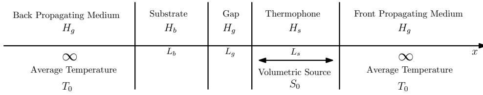
Figure 12: Schematic of a thermophone placed on a solid substrate of finite thickness on the left, and radiating in free field on the right. The plane waves are non-symmetrically generated within the back and the front media.
