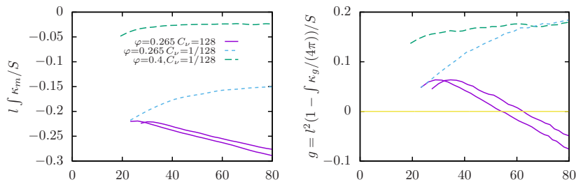
FIG. 10. Evolution with characteristic length of the mean curvature (left) and rescaled genus (right) for the same volume fraction \varphi = 0.265 (and \varphi = 0.4 , C_\nu = 1/128 as a visual reference) and different values of the viscosity ratios. The values interpolated from the fit of the self-similar regime close to the perfectly symmetric point are: \kappa_m = -0.18 , -0.10 , g = 0.20 , 0.06 when C_\nu = 128, 1/128 .
