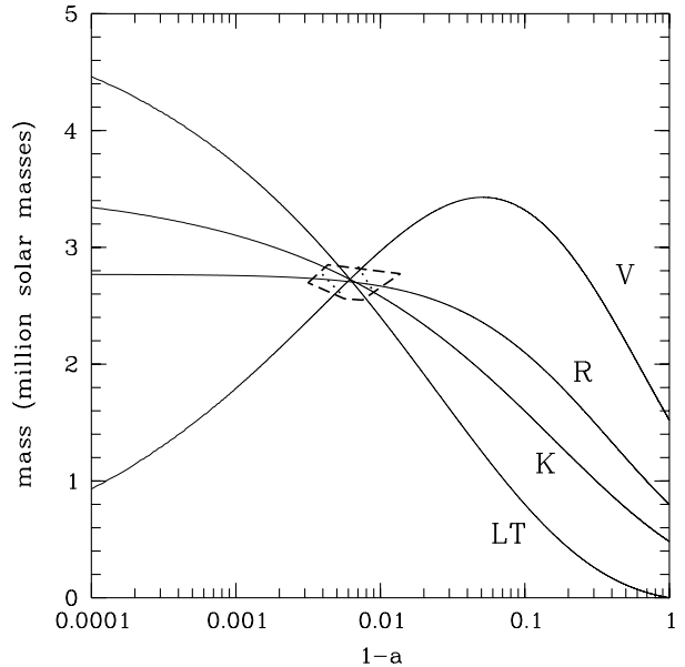
Fig. 7. Relation of M_{\text{BH}} versus (1-a) . Each curve represents one period assigned to a specific gravitational mode, coded by a label described in the text. The error region is enclosed by the dashed polygon. The dotted polygon is narrower because of the additional constraints imposed by the 321 s period (LT).
