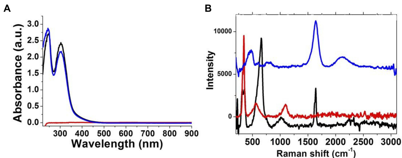
Figure 1 (A) UV-Vis absorption of \text{HAuCl}_4 \cdot 3\text{H}_2\text{O} (black line), \text{GdCl}_3 \cdot 6\text{H}_2\text{O} (red line); Au-Gd complex (blue line) in the range 200–900 nm (B) Raman spectra of Gd@Au complex (blue line) in the range 200–3000 \text{cm}^{-1} , compared to \text{HAuCl}_4 \cdot 6\text{H}_2\text{O} (black line), \text{GdCl}_3 \cdot 6\text{H}_2\text{O} (red line) as controls. Experimental conditions: \lambda_{\text{exc}} = 785 \text{ nm} ; laser power 20 mW; accumulation time 180 s.
