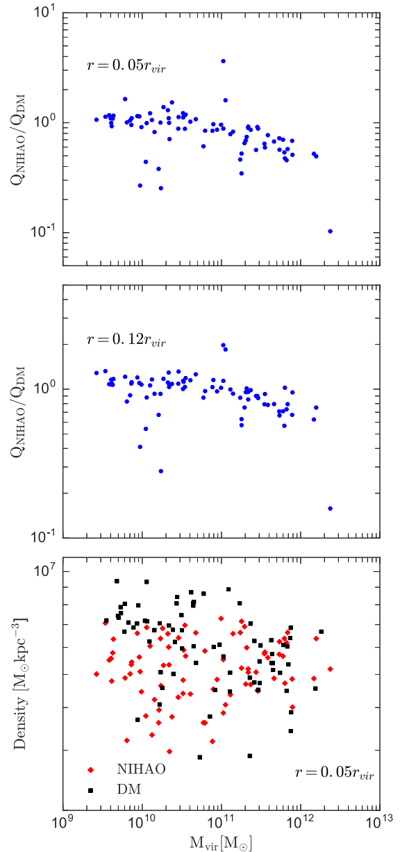
Figure 13. The top panel shows the ratio of the values of Q in the dissipationless and hydro simulations computed at 0.05 R_{\text{vir}} ( 0.12 R_{\text{vir}} for the middle panel). The outliers in the plot are due to merging galaxies (haloes) which are at a slightly different merging state in the hydro and DM simulations. The bottom panel shows the values of \rho at 5 per cent of R_{\text{vir}} for the DM (black) and the NIHAO (red) simulations.
