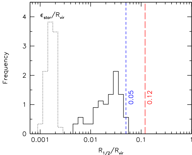
Figure 2. Histogram of the ratio between stellar half-mass radius, R_{1/2} , and the virial radius, R_{\text{vir}} . For reference, the three radii at which we will compute the halo shape are: R_{\text{vir}} , 12 per cent R_{\text{vir}} (red line) and 5 per cent R_{\text{vir}} (blue line). The leftmost histogram shows the distribution of the stellar particle softening through NIHAO.
