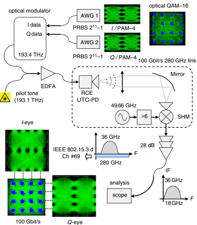
Fig. 1 100 Gbit/s wireless link. Carrier frequency 280 GHz, up to 25 GBaud QAM-16 modulation scheme. Emitter: RCE UTC-PD and receiver: SHM. The THz modulated 100 Gbit/s signal falls in channel 69 (252.72–321.4 GHz) of IEEE standard 802.15.3d [1]
