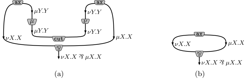
Fig. 5: Graph of \mu\text{MLL}^\infty proof structures
