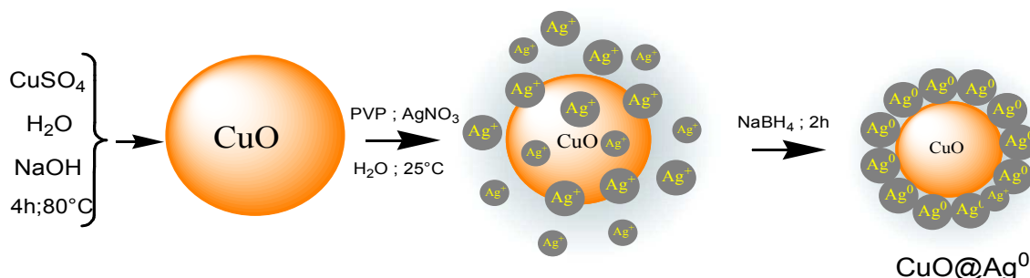
Scheme 1. Synthetic route for \text{CuO}@\text{Ag}^0 core-shell.
