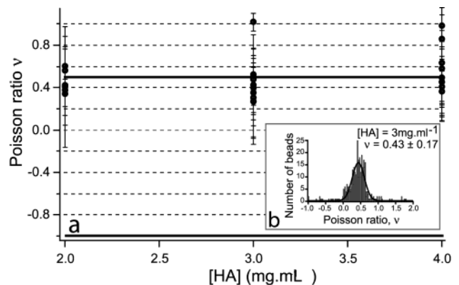
Figure 5. Poisson ratios, \nu (a), measured for three HA gels of different concentrations. The inset b shows an example of a Gaussian fit (full line) to the distribution of \nu obtained for a 3 mg ml -1 gel by analyzing the deflection of the colloidal bead with eq 4. The circles and error bars given in panel a are, respectively, the mean values and the standard deviations given by the Gaussian fits.
