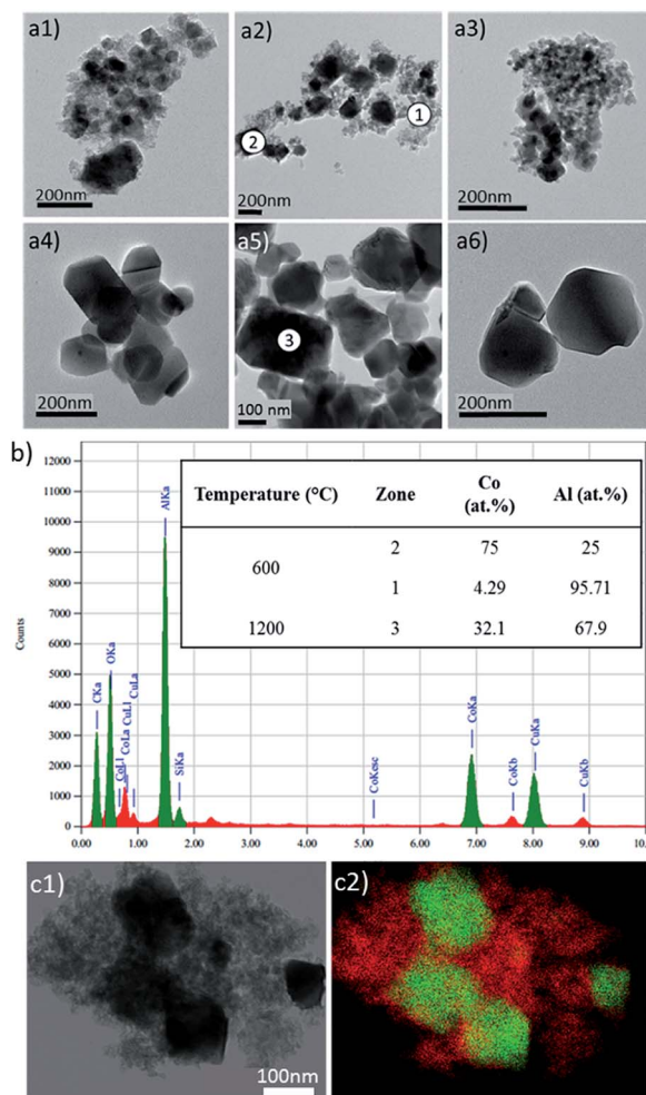
Fig. 2 (a) TEM micrographs of powders calcined at (a1) 400 °C, (a2) 600 °C, (a3) 800 °C, (a4) 1000 °C, (a5) 1200 °C and (a6) 1400 °C. (b) EDX results on the different areas indexed on the micrographs, (c) TEM micrograph (c1) and the corresponding chemical cartography (c2) showing for the 600 °C-annealed compound the non-homogeneous distribution of cobalt and aluminium ions (red colour: Al, green colour: Co).
