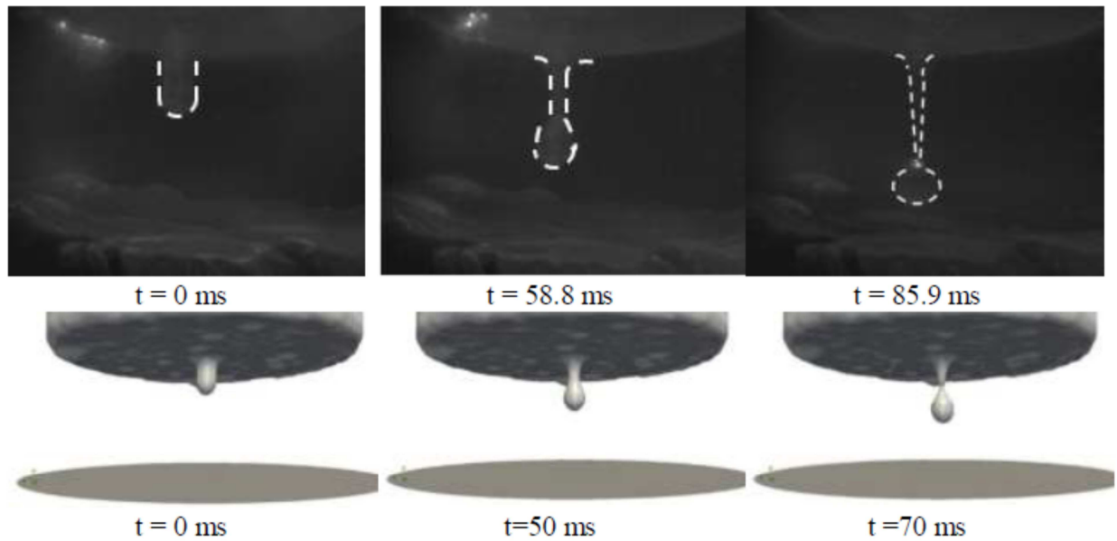
Figure 4. Formation and detachment of a drop observed experimentally (top row) and predicted by the numerical model (bottom row).
