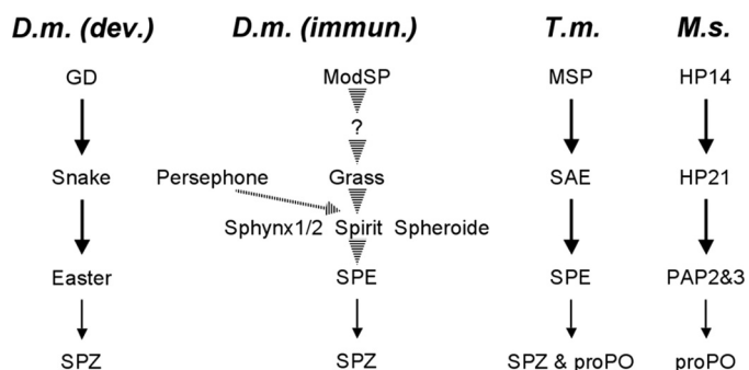
FIGURE 1. Current knowledge of the proteolytic cascades involving clip-SPs, as described in the literature. The figure depicts the proteolytic cascades of the development and immunity. Left , development in D. melanogaster ( D.m. dev. ) (3). Center , immunity in D. melanogaster ( D.m. immun. ) (8, 9). Right , immunity in T. molitor ( T.m. ) (12) and in M. sexta ( M.s. ) (15). Arrows indicate experimentally verified direct links. Dashed arrows indicate steps that have not been experimentally verified or in which components of the pathway have not been identified.
