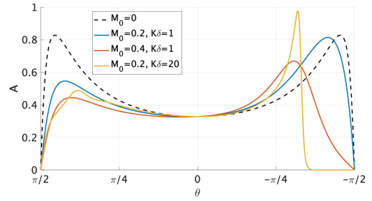
FIG. 5. (color online) Value of the absorption coefficient A as a function of \theta for several flows, described by their mean Mach number M_0 and the height of their shear layer \delta for a liner of admittance Y = 0.1i - 0.1 .
