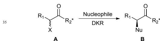
Scheme 1 Dynamic kinetic resolution of \alpha -halo carbonyls by S_N2 halogen displacement.
