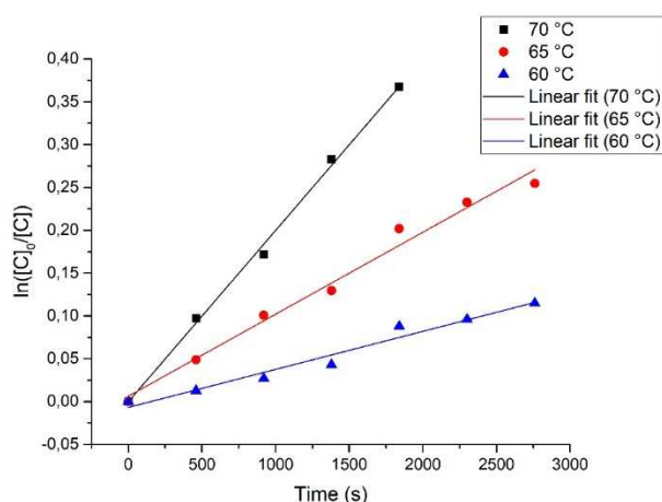
Figure 1. First order decay of [\text{Mn}(\text{CHMeCOOMe})(\text{CO})_5] ( 1 ) in \text{C}_6\text{D}_6 at 70, 65 and 60 °C in the presence of TTMSS.
