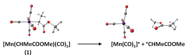
Figure 3. Views of the optimized geometries of [\text{Mn}(\text{CH}(\text{CH}_3)\text{COOCH}_3)(\text{CO})_5] ( 1 ), [\text{Mn}(\text{CO})_5]^\cdot and ^\cdot\text{CH}(\text{CH}_3)\text{COOCH}_3 , and DFT-calculated thermochemical parameters.
