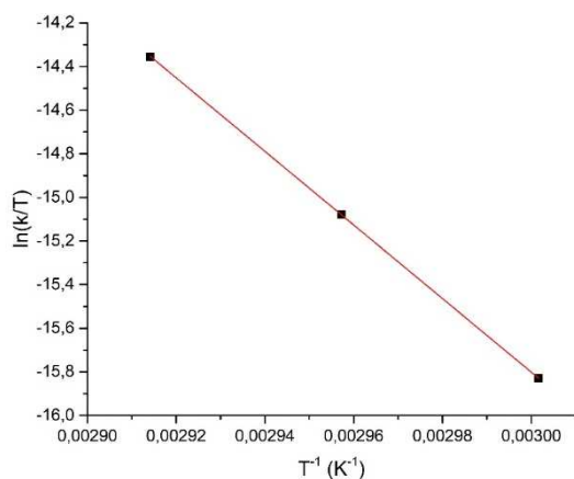
Figure 2. Eyring plot of k_{\text{obs}} as function of temperature for the decomposition of compound 1 .
