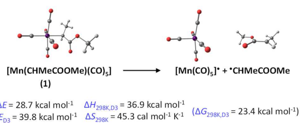
Figure 3. Views of the optimized geometries of [\text{Mn}(\text{CH}(\text{CH}_3)\text{COOCH}_3)(\text{CO})_5] ( 1 ), [\text{Mn}(\text{CO})_5]^\cdot and ^\cdot\text{CH}(\text{CH}_3)\text{COOCH}_3 , and DFT-calculated thermochemical parameters.
