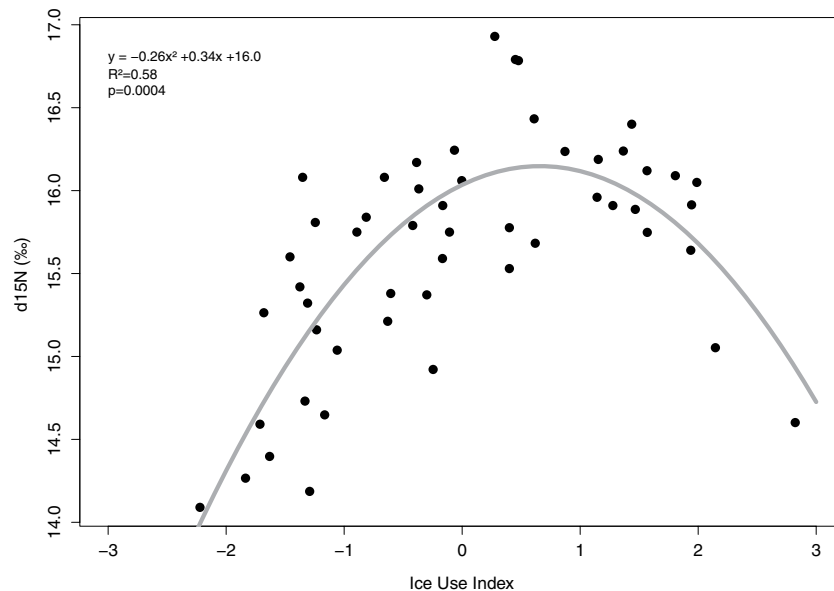
Figure 4. Influence of ice association (ice use index) on \delta^{15}\text{N} ratios measured in eggs of thick-billed murre between 2010 and 2013.
