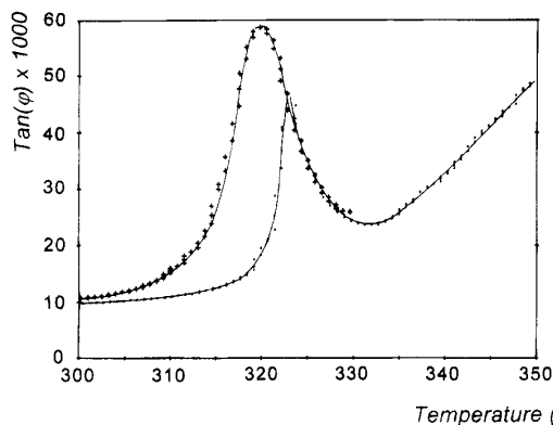
Figure 3. Isochronal spectra (1 Hz) measured on heating showing the effect of reversible physical aging at room temperature and rejuvenation on quenching: (●) after aging at room temperature; (+) second run after fast cooling from 350 K.
