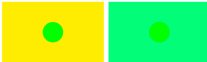
Figure 2: The inner disks appearing in the center of the two images are exactly the same physical color stimulus. However, the one in the left image is perceived, with respect to its background illumination, as a very saturated green, instead, after the change of background illumination shown by the image on the right, the color stimulus is perceived as yellowish. Due to the small size of the color stimuli on this document, they are surrounded by a thin black circle to enhance their visibility.
