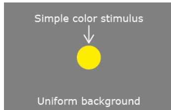
Figure 1: In Resnikoff's model a color is always associated to a couple given by a physical light and a uniform background illumination in which it is embedded.
