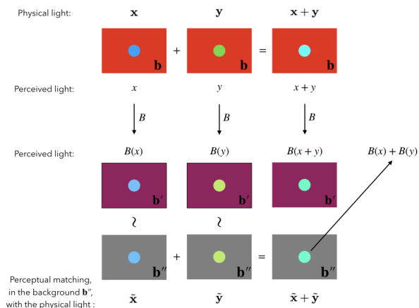
Figure 4: The experimental setup outlined in the picture can be used to check the additivity of background transformations, see the text for a detailed description.
