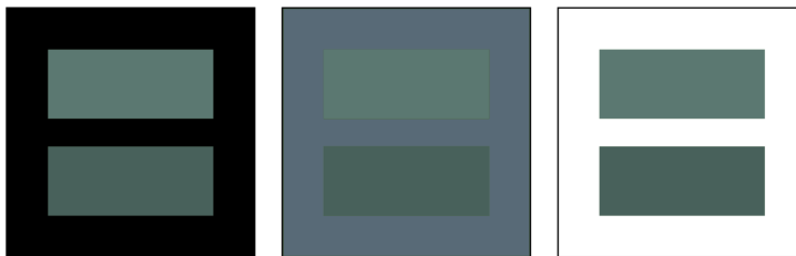
Figure 5: The crispning effect (see text) used to refute Resnikoff's Axiom 6 about the invariance of the perceptual color metric with respect to changes of background illuminations.
