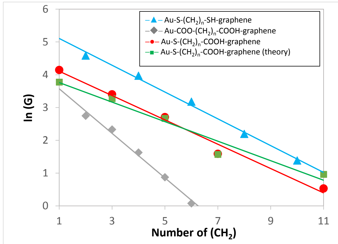
Figure 5 : Natural logarithmic plots of the conductance as a function of the number of methylene groups for Au-S-(CH 2 ) n -SH-graphene (blue), Au-COO-(CH 2 ) n -COOH-graphene (grey), Au-S-(CH 2 ) n -COOH-graphene (red) and Au-S-(CH 2 ) n -COOH-graphene (theory, green)
