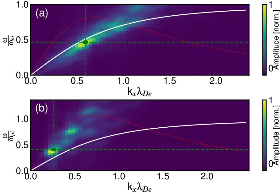
Figure 8: 2D FFT of the azimuthal electric field at x=0.3 cm (a) and x=1.5 cm (b), obtained with code LPP . Solid white line: ion acoustic dispersion relation. Red pointed line: growth rate of ion acoustic instability (rescaled). Green dashed lines: wavelength and frequency of the dominant mode.
