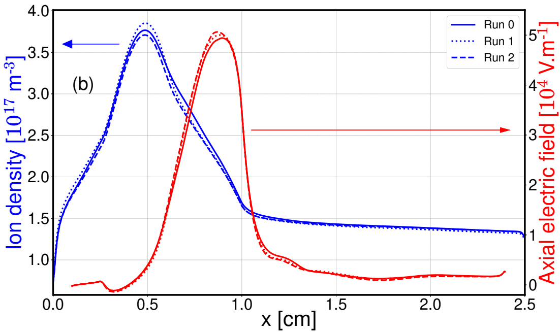
Figure 12: Comparison of 3 simulations with the same code ( LPP ) for the same input parameters (Case 2). (a): Time evolution \frac{J_{ec1}}{J_M} . (b): Azimuthally and time (between 11 and 15 \mu\text{s} as represented by the two vertical dashed lines of (a)) averaged profiles of ion density (blue) and axial electric field (red).
