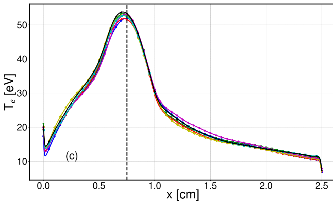
Figure 7: Case 3 : Azimuthally and time (between 16 and 20 \mu\text{s} ) averaged axial profiles of axial electric field (a), ion density (b) and electron temperature (c). Dashed line corresponds to the position of maximum magnetic field.
