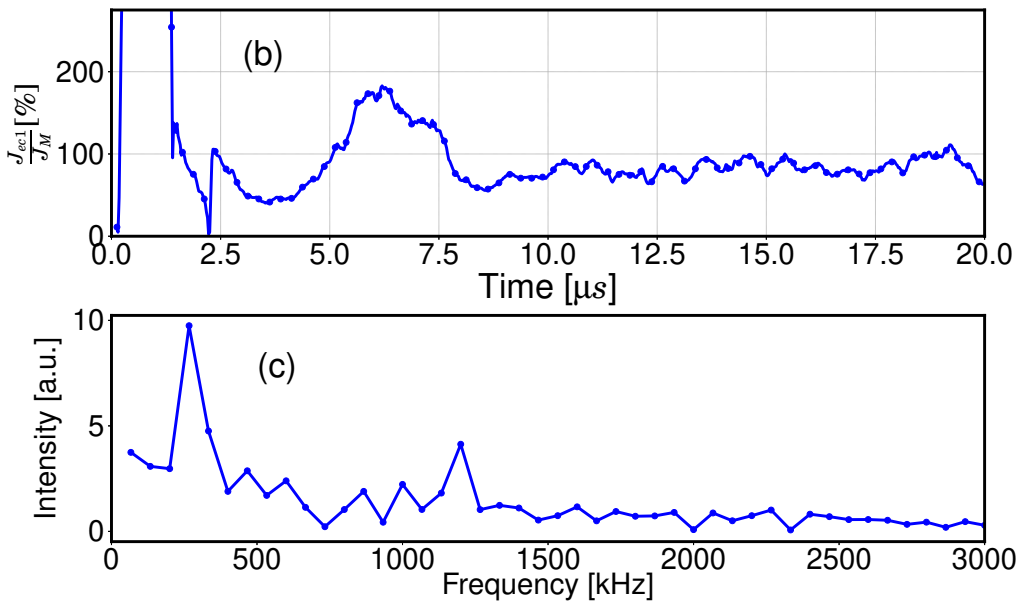
Figure 3: (a) : Time evolution of \frac{J_{ec1}}{J_M} for Case 1 for all the codes. Brown dashed line: beginning of time averaging interval (until 20 \mu\text{s} ). (b): Time evolution of \frac{J_{ec1}}{J_M} for Case 1 with code LPP . (c): Corresponding Fast-Fourier-Transform taken from data between 12 and 20 \mu\text{s} .
