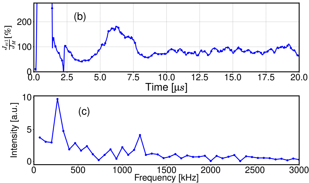
Figure 3: (a) : Time evolution of \frac{J_{ec1}}{J_M} for Case 1 for all the codes. Brown dashed line: beginning of time averaging interval (until 20 \mu\text{s} ). (b): Time evolution of \frac{J_{ec1}}{J_M} for Case 1 with code LPP . (c): Corresponding Fast-Fourier-Transform taken from data between 12 and 20 \mu\text{s} .
