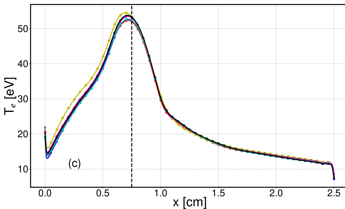
Figure 6: Case 2 : Azimuthally and time (between 16 and 20 \mu\text{s} ) averaged axial profiles of axial electric field (a), ion density (b) and electron temperature (c). Dashed line corresponds to the position of maximum magnetic field.
