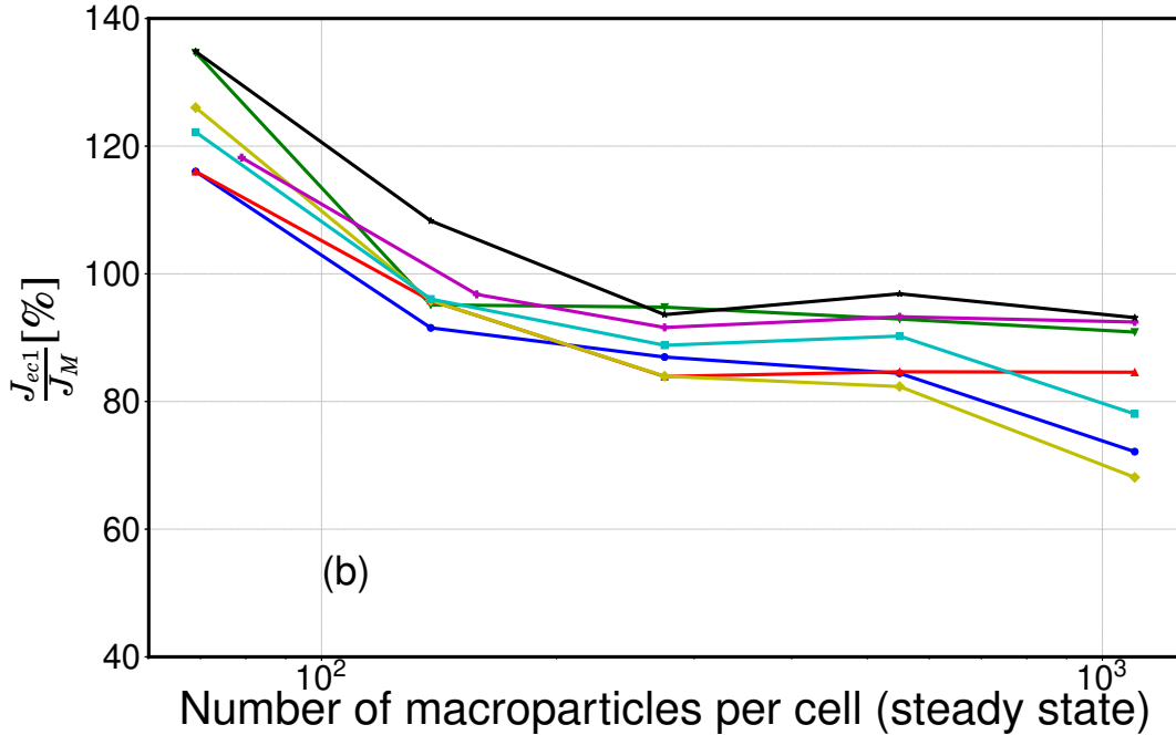
Figure 11: Mean value (between 12 and 20 \mu s) of \frac{J_{ecl}}{J_M} depending on N_{ppc,final} in normal scale (a) and semi-log scale (b). The three benchmark cases correspond to N_{ppc,final} = 550 (Case 1), N_{ppc,final} = 275 (Case 1) and N_{ppc,final} = 1100 (Case 3).
