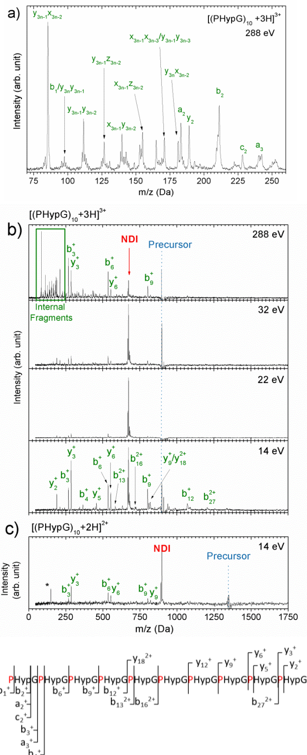
Figure 3 Photoabsorption mass spectra of [(\text{PPG})_{10}+3\text{H}]^{3+} at 14, 22, 32 and 288 eV (b) and of [(\text{PPG})_{10}+2\text{H}]^{2+} at 14 eV (c). The position of the precursor ion is indicated by dots,
