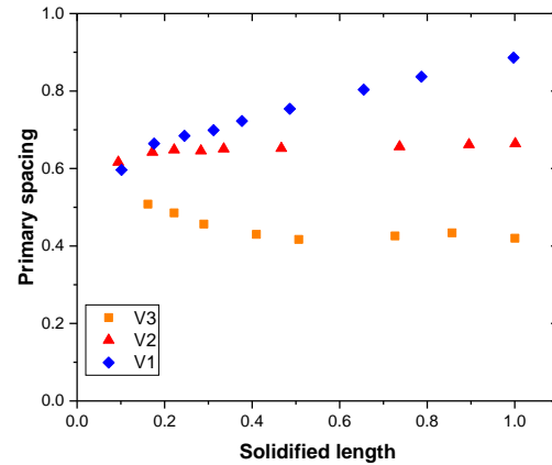
Fig. 4. Primary spacing evolution as a function of the solidified length for different pulling rates ( V_3 > V_2 > V_1 ).
