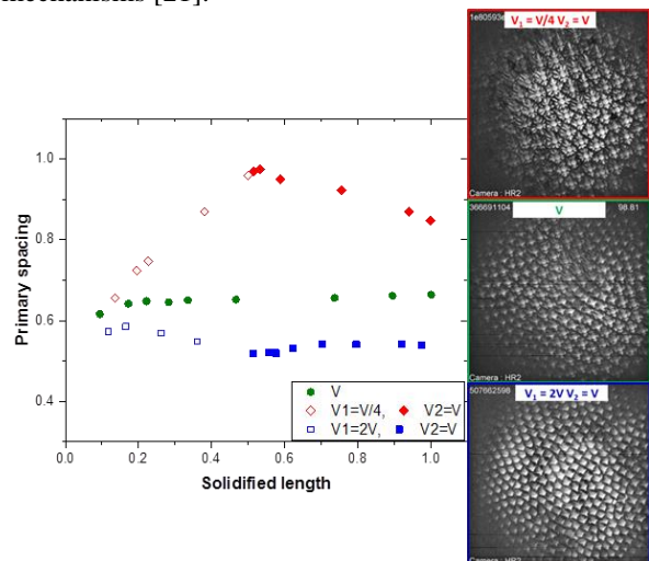
Fig. 7. Primary spacing evolution at V from rest ( \bullet ), after half-way solidification at V/4 ( \blacklozenge, \blacklozenge ) or 2V ( \blacksquare, \square ). Axial view snapshots at the end ( 7.3 \times 7.3 \text{ mm}^2 ). The primary spacing and the solidified length were normalized similarly to fig. 4.
