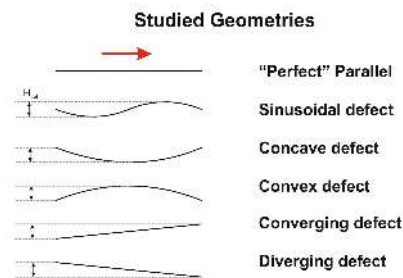
Fig. 1 Geometrical imperfection of fluid pad interface.
