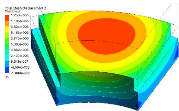
Fig. 4 Mesh displacement of the pad domain of a perfect parallel thrust bearing
