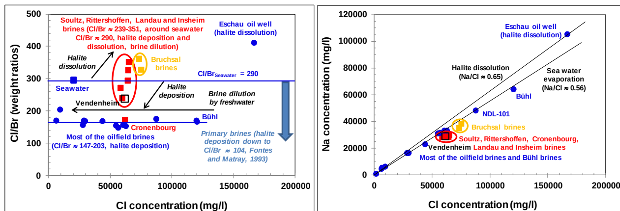
Figure 5: Binary diagrams Cl/Br-Cl and Na-Cl for the most representative deep brine of the Vendenheim wells.
