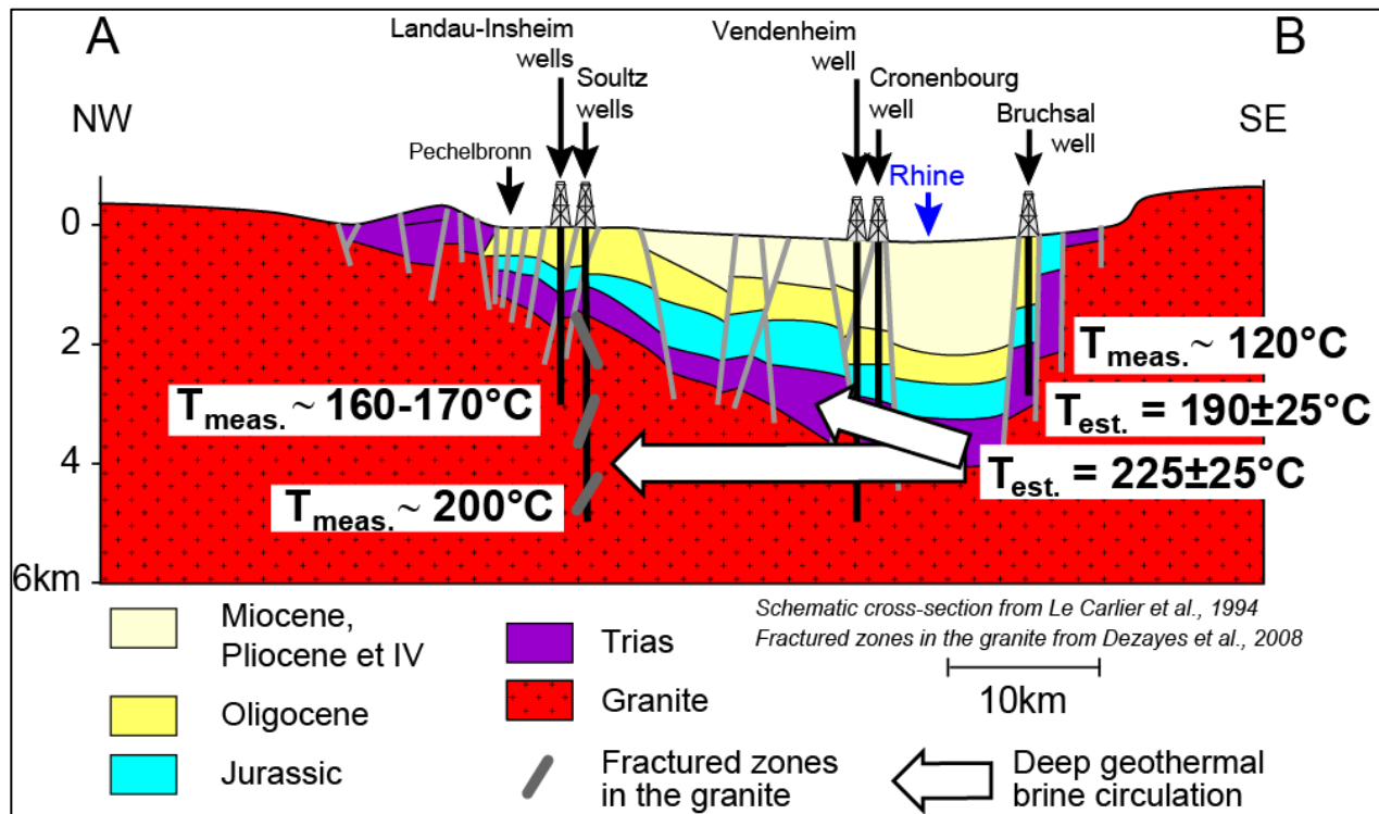
Figure 9: Schematic NW-SE cross-section of the Upper Rhine Graben in which several deep wells (Bruchsal - Cronenbourg, near Vendenheim - Landau - Insheim - Soultz) drilled to depths between 2450 and 5000 m have been reported (from Le Carlier et al. , 1994; Dezayes and Genter, 2008; Sanjuan et al. , 2010; 2016a).
