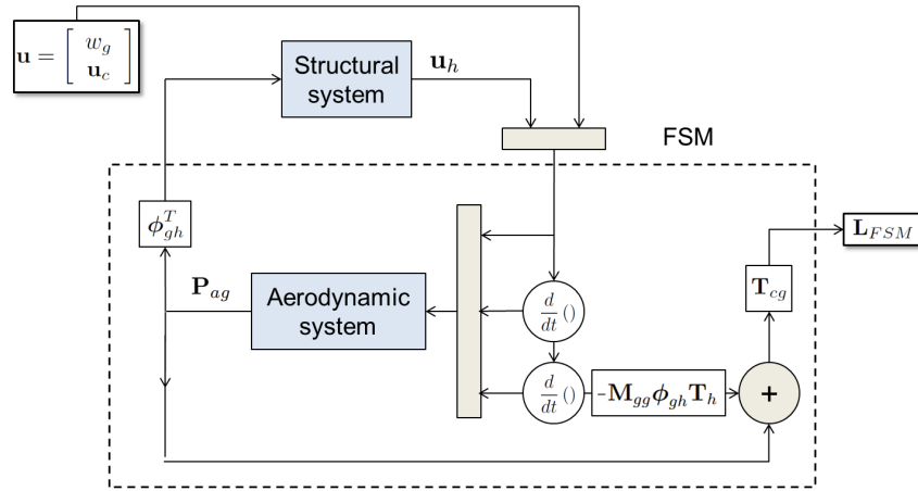
Figure 4: Aeroservoelastic system with the force summation method (FSM) for the cut loads recovery.
