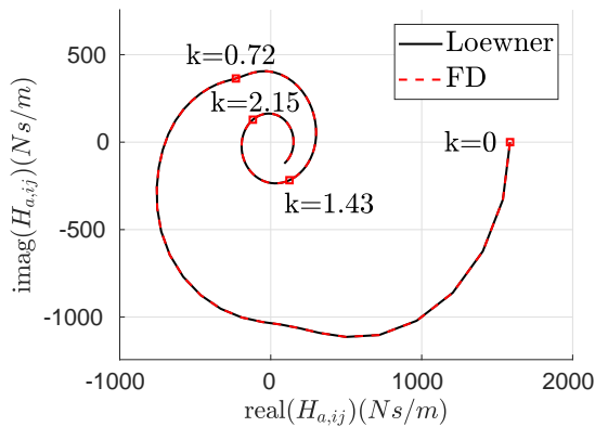
Figure 15: Element of the aerodynamic transfer function matrix from the gust input to the the vertical force for a node at position x = 30.1076 (m), y = 3.6521 (m), z = 3.9362 (m).
