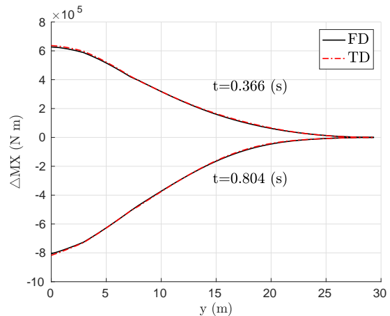
Figure 9: Incremental bending moment \Delta MX over the right wing component at different time instants for M_\infty = 0.86 , h = 9100 (m), H = 50 (ft), \alpha_{eq} = 1 (deg). Results obtained in the frequency domain (FD) and with the generalized state-space model in the time domain (TD) by the FSM with 16 flexible modes. The number of states is 231.
