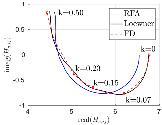
Figure 7: Element of the transfer function matrix from the pitch input to the lift coefficient for the strip at wing station y = 13.48 (m).
