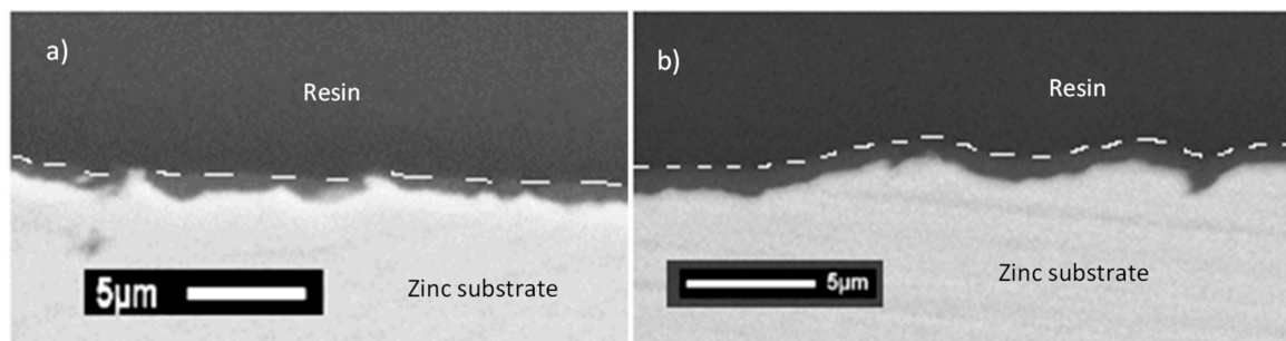
Figure 3. Scanning electron micrographs of cross-section of coatings deposited on natural zinc: (a) TEOS/MAP, and (b) GPTMS/ASB.
