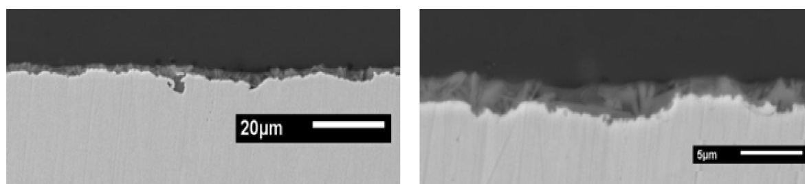
Figure 11. Scanning electron micrographs of cross-section of TEOS/(50%MAP + 50%UPS) coating deposited on phosphated zinc.
