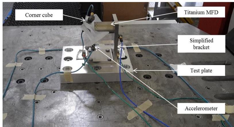
Figure 4: Corner cube on the electrodynamic shaker for sine test
