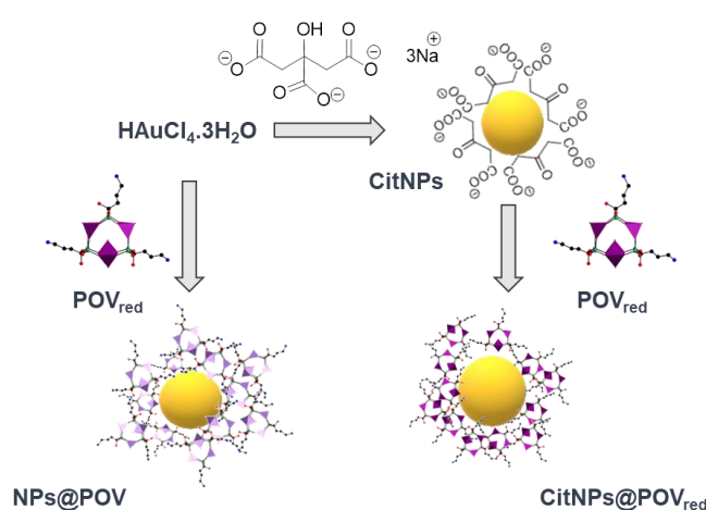
Scheme 1: Schematic representation of CitNPs, CitNPs@ \text{POV}_{\text{red}} and NPs@POV synthesis.
