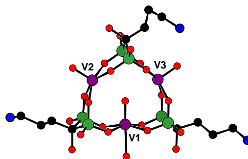
Fig. 1: Ball-and-stick representation of one of the molecule present in the structure of the \text{V}_3(\text{Ale})_3 complex. Purple sphere = V, green spheres = P, black spheres = C, red spheres = O, blue spheres = N; H atoms were omitted for clarity.
