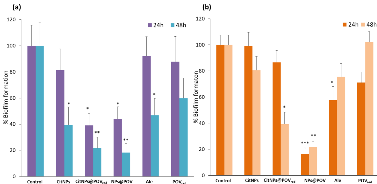
Fig. 3: The effect of CitNPs (1.3 nM), CitNPs@POV red (1.3 nM), NPs@POV (1.0 nM), alendronate (540 \mu M), and POV red (180 \mu M) on biofilm formation by (a) P. aeruginosa and (b) S. epidermidis after incubation for 24 and 48 h in 96-well plates. The values of the experimental groups were compared with the control group. Statistical significance was analyzed by Student's T-test to detect the presence of statistically significant differences (*** p<0.001, **p<0.01, *p<0.05)***) For CitNPs, CitNPs@POV red and NPs@POV the numbers in brackets correspond to the concentration in gold nanoparticles
