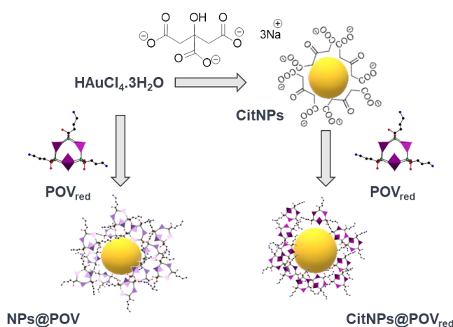
Scheme 1: Schematic representation of CitNPs, CitNPs@ \text{POV}_{\text{red}} and NPs@POV synthesis.
