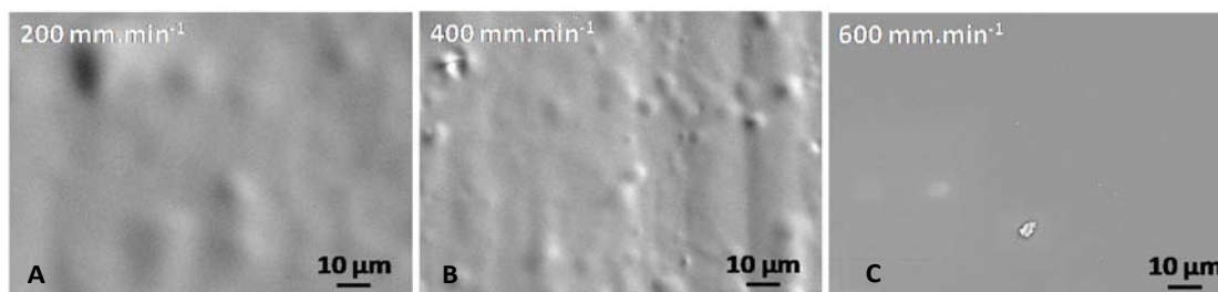
Figure 9. Coating surface micrographs for bilayer systems by SEM performed for deposits with various withdrawal speeds (A) 200 \text{ mm} \cdot \text{min}^{-1} ; (B) 400 \text{ mm} \cdot \text{min}^{-1} and (C) 600 \text{ mm} \cdot \text{min}^{-1} .
