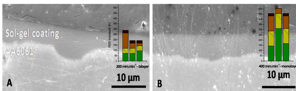
Figure 12. Comparison between (A) bilayer and (B) monolayer system (similar thickness).
