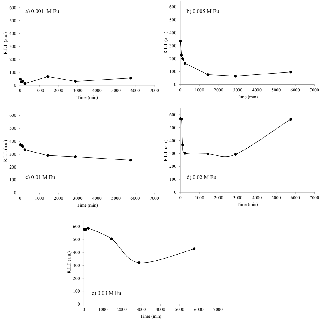
Figure SI3. Effect of the precipitation time over the R.L.I. of the different \text{Eu}^{3+} doping concentrations. \lambda_{\text{exc/em}} = 394/614 nm, slit-widths exc/em = 5/5 nm, t_d = 0.120 \mu\text{s} , t_g = 5 ms and detector voltage = 500 v.
