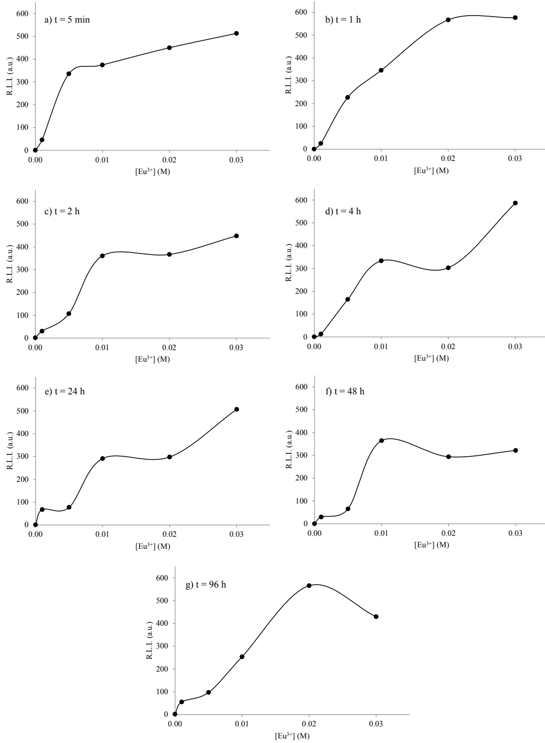
Figure SI4. Effect of the \text{Eu}^{3+} doping concentration over the R.L.I. of the different materials precipitated at different times. \lambda_{\text{exc/em}} = 394/614 nm, slit-widths exc/em = 5/5 nm, t_d = 0.120 \mu\text{s} , t_g = 5 ms and detector voltage = 500 v.
