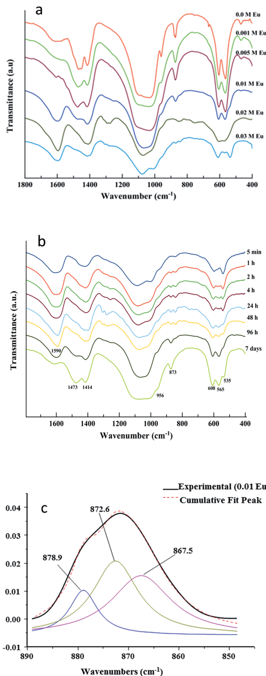
Fig. 4 FTIR spectra of samples prepared: (a) in the presence of \text{Eu}^{3+} doping concentrations from x = 0.00 to 0.030 M, at 96 hours and (b) for x = 0.010 M \text{Eu}^{3+} at maturation times between 5 min to 7 days. (c) Detailed FTIR analysis of the \nu_3\text{CO}_3 region for sample prepared in presence of 0.01\text{ M Eu}^{3+} at 96 h maturation.
