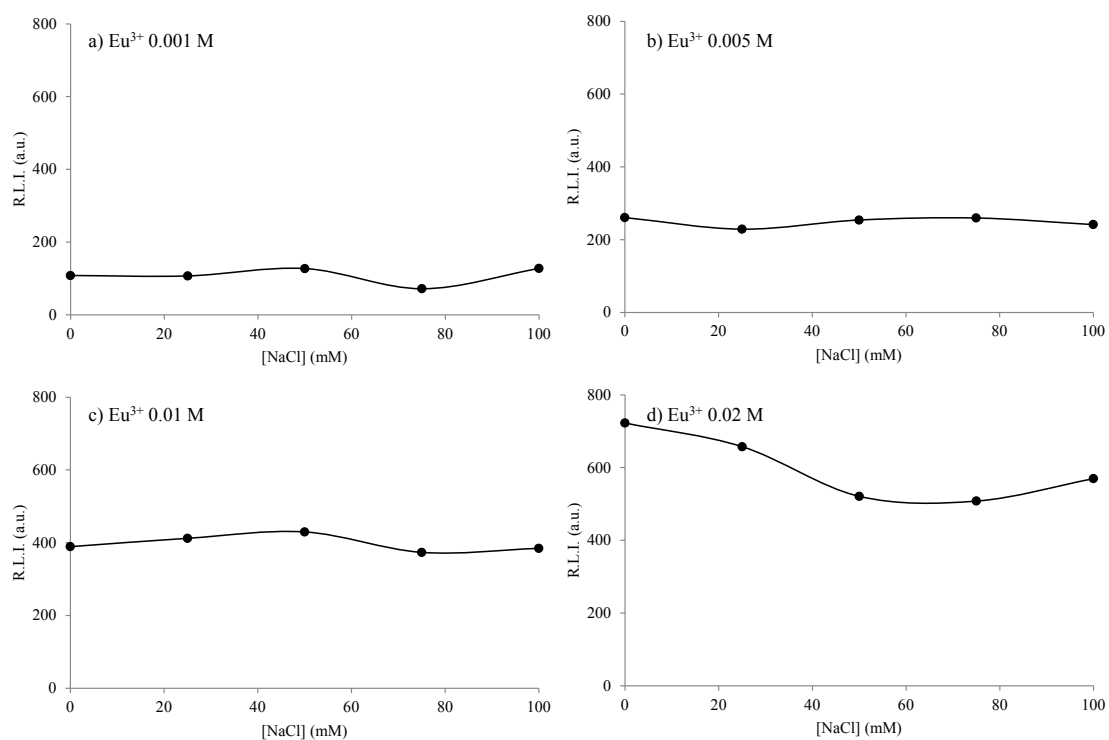
Figure SI6. Effect of the ionic strength on the luminescence of the different \text{Eu}^{3+} doping concentrations dispersed in aqueous solution at pH=7.0 and 25°C. \lambda_{\text{exc/em}} = 232/616 nm, slit-widths exc/em = 10/10 nm, t_d = 0.120 \mu\text{s} , t_g = 5 ms and detector voltage = 600 v.
