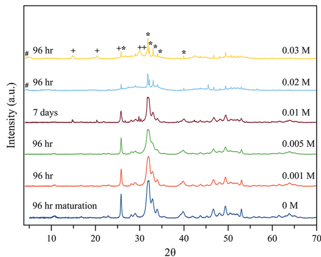
Fig. 2 XRD patterns of samples precipitated at 96 hours in the absence ( x = 0 ) and the presence of \text{Eu}^{3+} ( x = 0.001, 0.005, 0.020 and 0.030 \text{ M} ) and at 7 days ( x = 0.01 \text{ M} ). # (OCP, 100, PDF 44-0778), * (apatite phase, PDF 01-1008), + ( \text{EuPO}_4 \cdot \text{H}_2\text{O} phase, PDF 20 1044).
