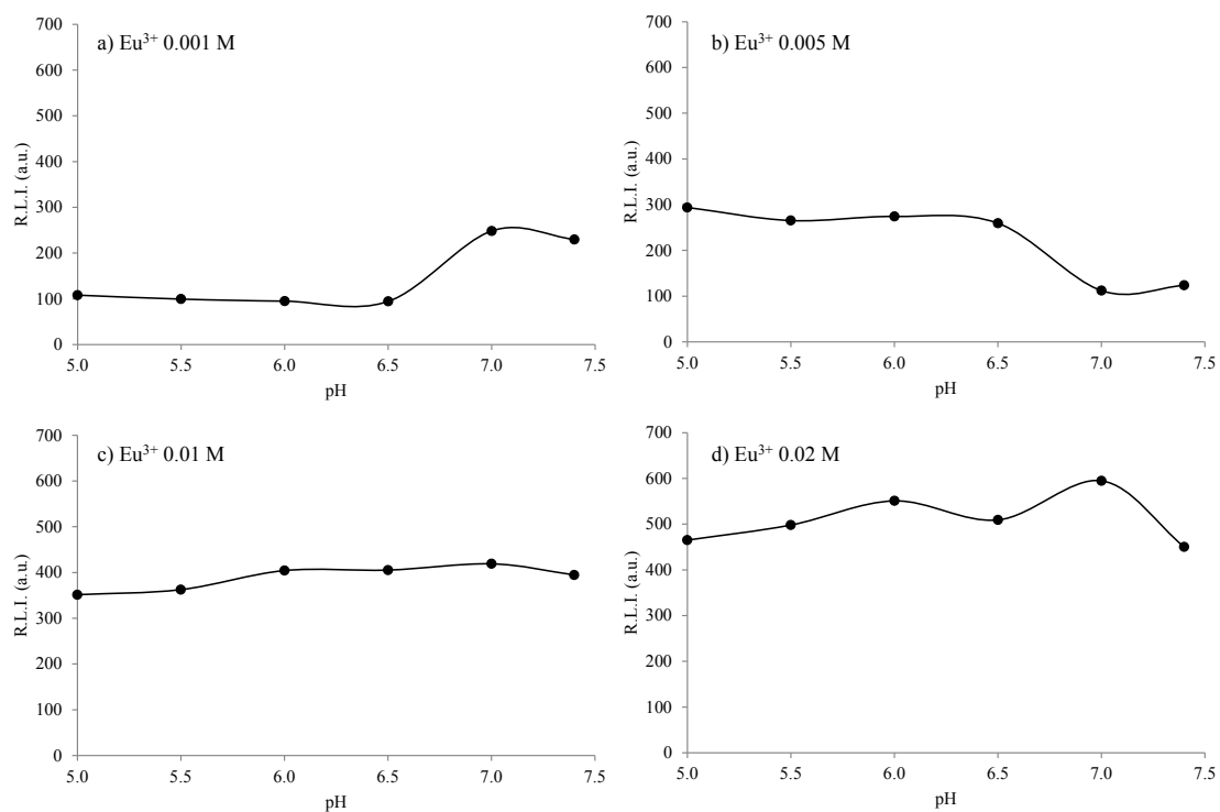
Figure SI5. Effect of the pH on the luminescence of the different \text{Eu}^{3+} doping concentrations dispersed in aqueous solution at 25°C. \lambda_{\text{exc/em}} = 232/616 nm, slit-widths exc/em = 10/10 nm, t_d = 0.120\mu\text{s} , t_g = 5 ms and detector voltage = 600 v.
