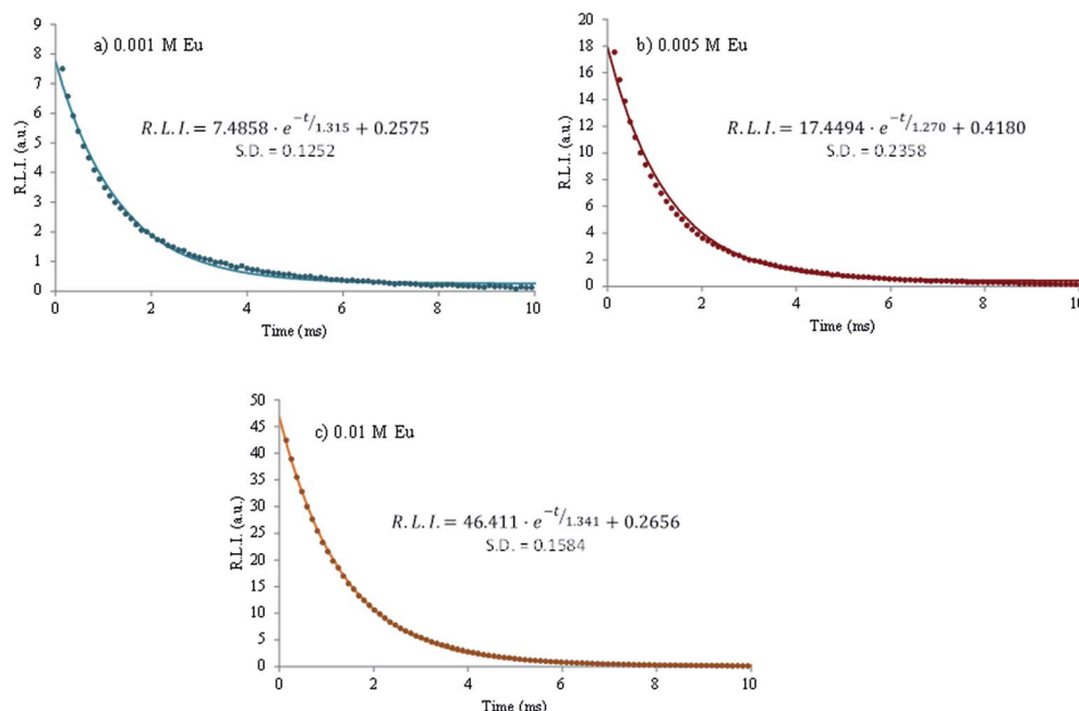
Fig. 8 Luminescence decay curve of Eu-doped cit-cAp prepared with different \text{Eu}^{3+} doping concentrations at maturation times of 96 h. \lambda_{\text{exc/em}} 394/614 nm, slit-widths exc/em 5/5 nm and detector voltage 550 V. Circles correspond to experimental data and lines to the fitting equation.
